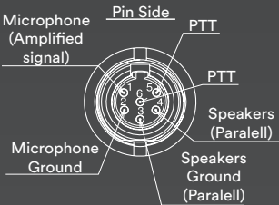
Pin Configuration for -111 Headset
