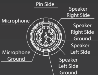
Pin Configuration for -110 Headset
